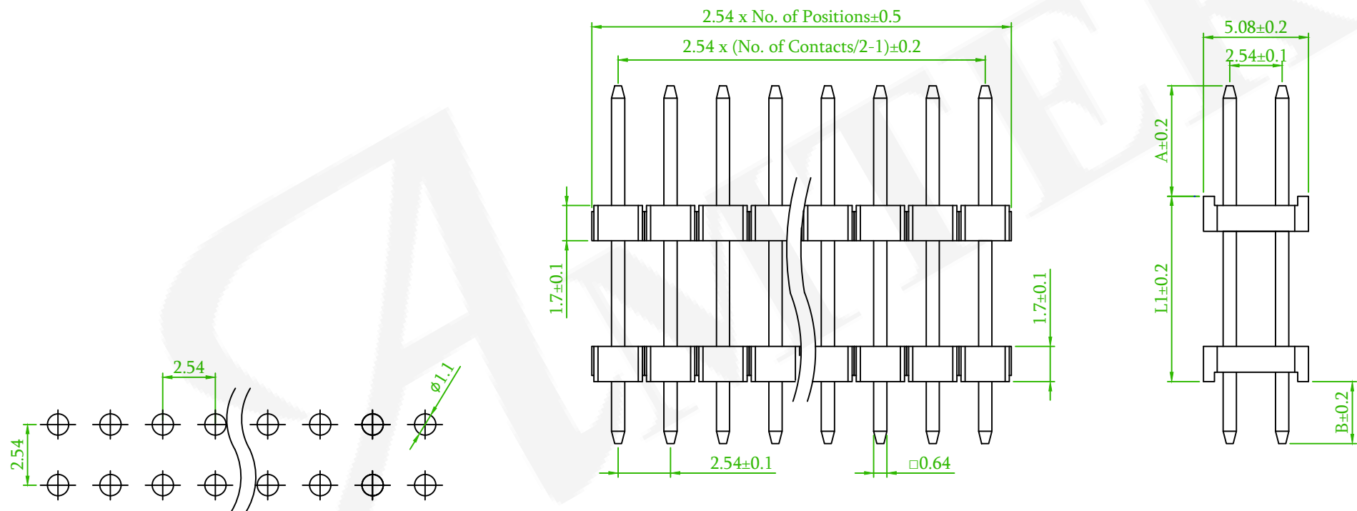
Recommended PCB Layout (PCB TOLERANCE ±0.1)
