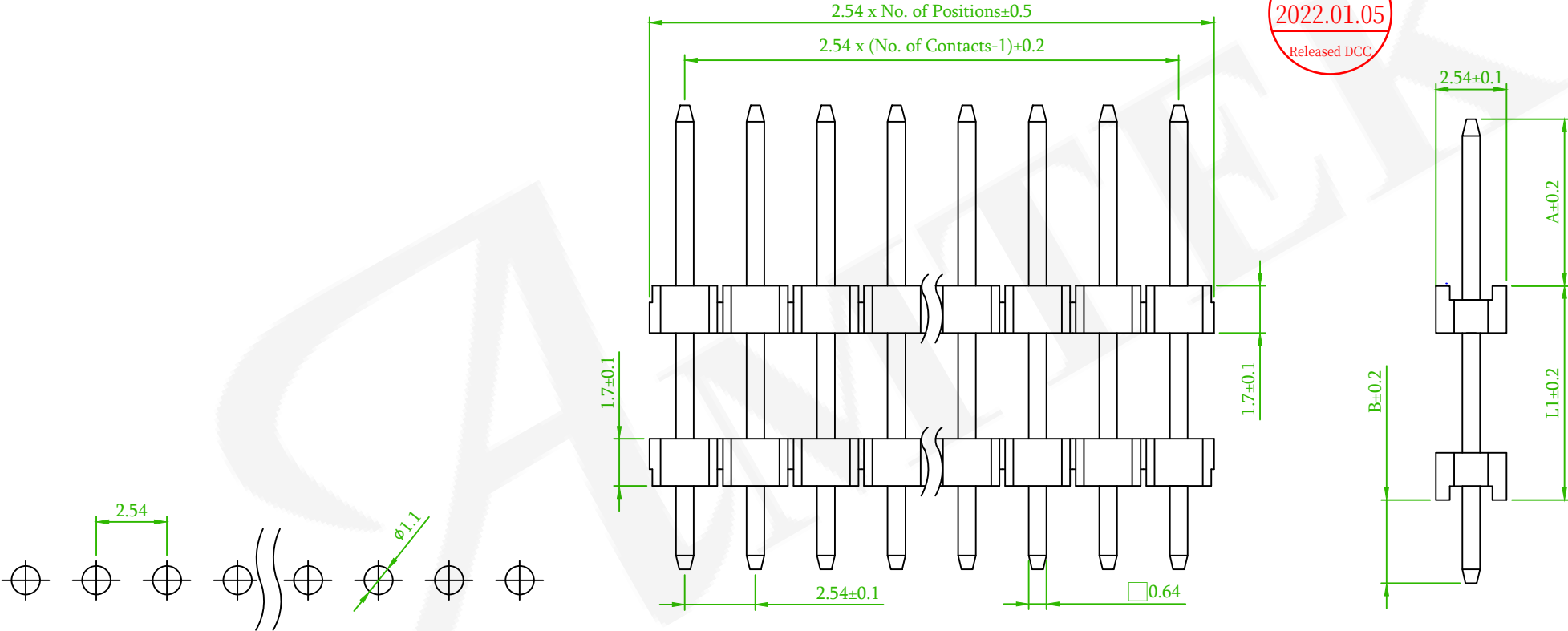
Recommended PCB Layout (PCB TOLERANCE ±0.1)
