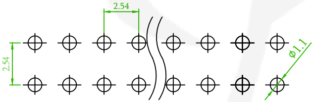
Recommended PCB Layout (PCB TOLERANCE ±0.1)
