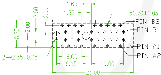
P.C.B LAYOUT COMPONENT SIDE
