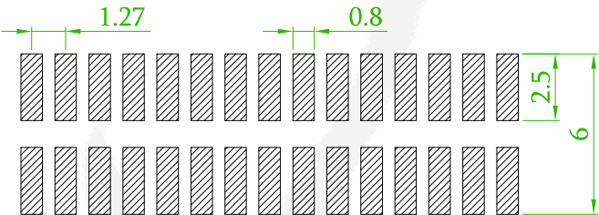
Recommended PCB Layout (PCB TOLERANCE ±0.05)
