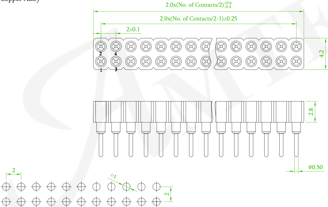
Recommended PCB Layout (PCB TOLERANCE ±0.05)
