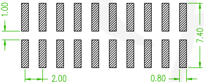
Recommended P.C.B Layout(Top Side) (PCB BOARD TOLERANCE±0.05)
