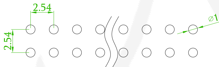
Recommended PCB Layout (PCB TOLERANCE ±0.1)
