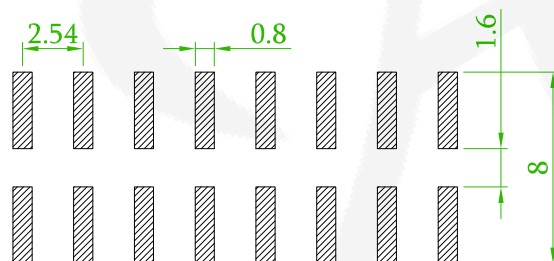
Recommended P.C.B Layout (PCB BOARD TOLERANCE \pm 0.1)
