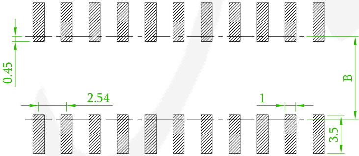
Recommended PCB Layout (PCB TOLERANCE±0.1)
