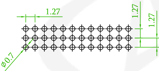
Recommended PCB Layout (PCB TOLERANCE ±0.1)
