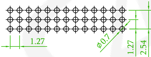
Recommended PCB Layout (PCB TOLERANCE ±0.1)
