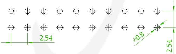
Recommended PCB Layout (PCB TOLERANCE ±0.05)
