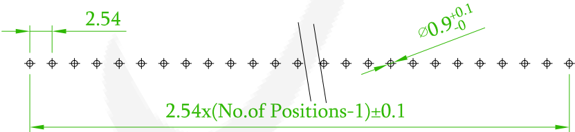
Recommended PCB Layout (PCB TOLERANCE ±0.1)
