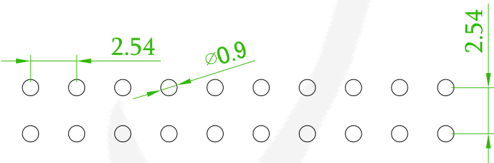
Recommended P.C.B Layout (PCB BOARD TOLERANCE±0.1)
