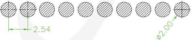
Recommended PCB Layout (PCB TOLERANCE ±0.1)
