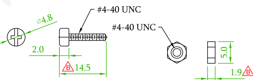
Short Screw
