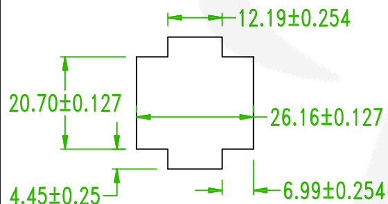
5H6350F0-303
