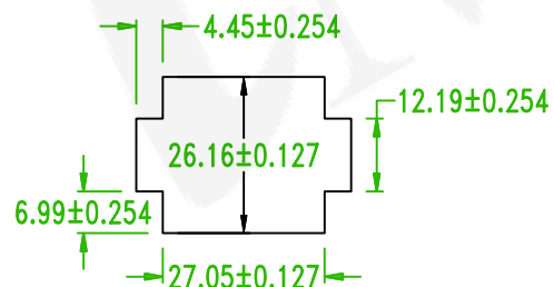
5H6350F0-304
