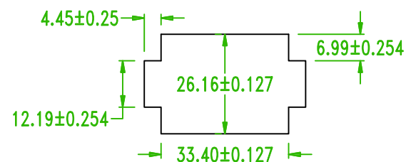
5H6350F0-305
