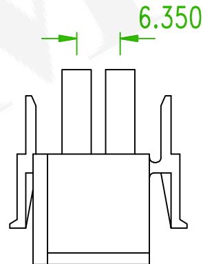
5H6350F0-302
