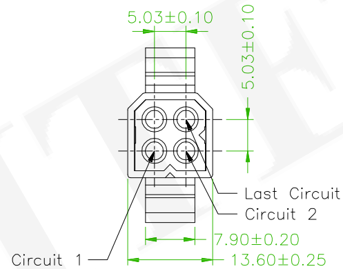
5H5030M1-202WBL00A01 2x2 Pin With Ear
