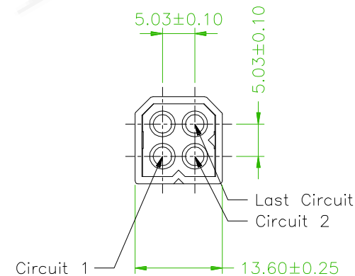
5H5030M0-202WBL00A01 2x2 Pin W/O Ear
