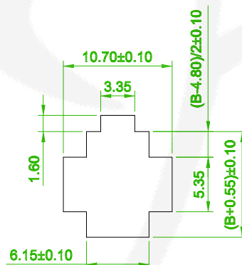
Panel hole layout (2P~3P)
