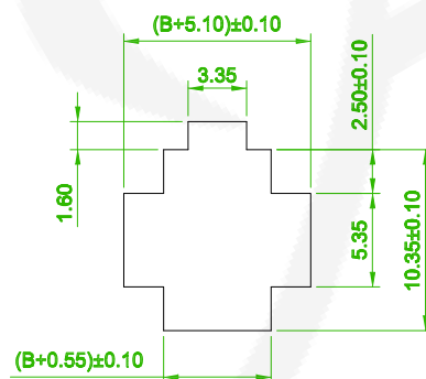
Panel hole layout
