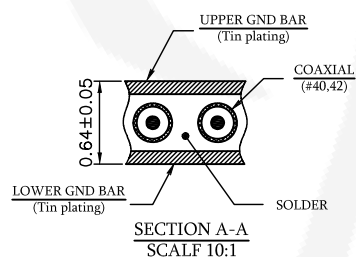
CABLE ASSEMBLED CONDITION(REF.)
