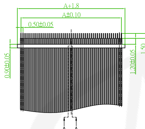
CABLE ASSEMBLED CONDITION(REF.)
