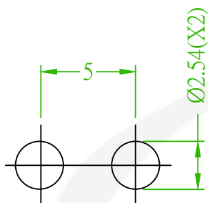
Mounting Hole
