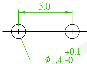
Mounting Hole
