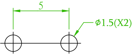
Mounting Hole
