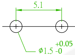
Mounting Hole
