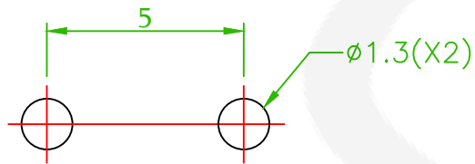
MOUNTING HOLE
