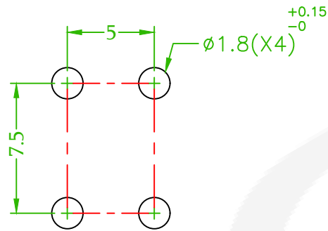
MOUNTING HOLES
