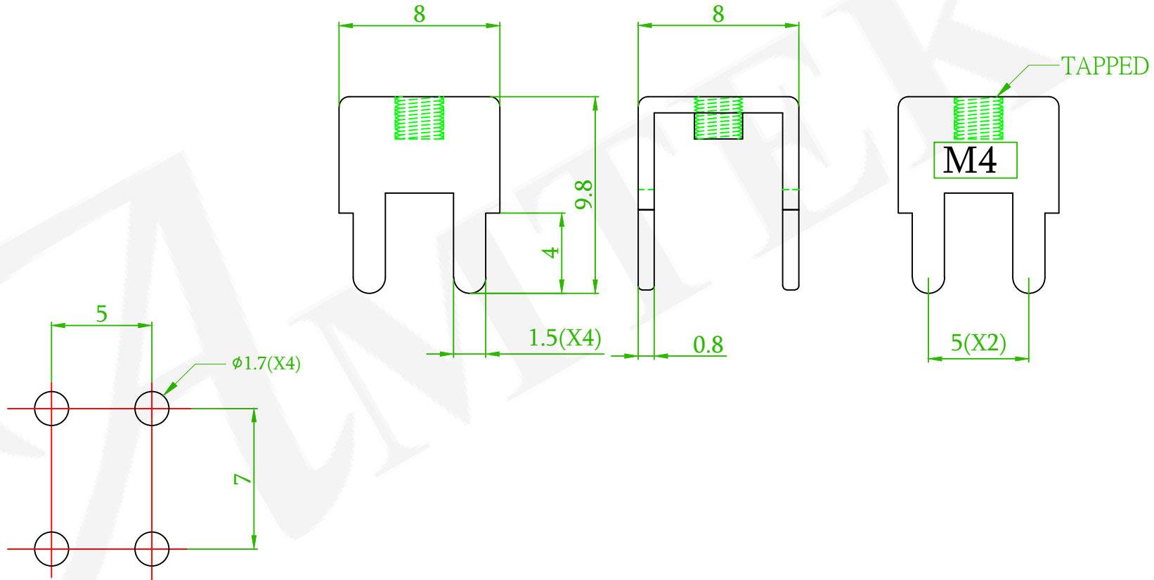
MOUNTING HOLE
