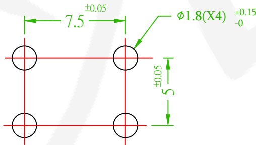
MOUNTING HOLES
