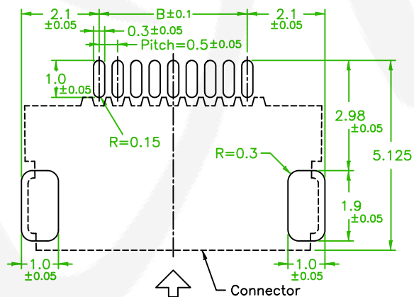
FPC/FFC INSERT DIRECTION Recommended PCB Board Hole Layout
