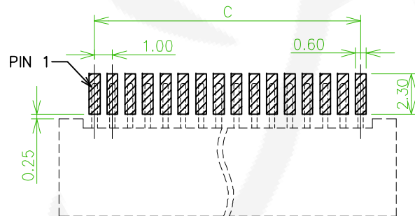
Recommended PCB Board Hole Layout
