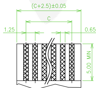
FPC/FFC T=0.30±0.05
