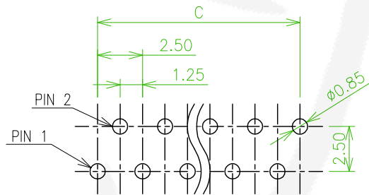
Recommended PCB Layout (PCB TOLERANCE \pm 0.05 )
