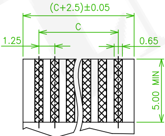
FPC/FFC T=0.30±0.05
