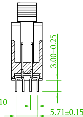
SECTION A-A Old Part No.:EDH4BS-XX-U
