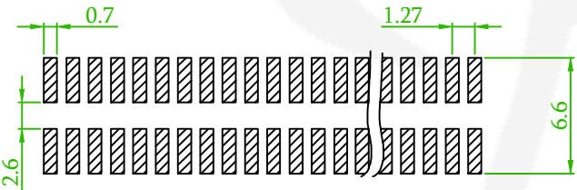
Recommended PCB Layout (PCB TOLERANCE ±0.05)
