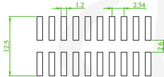
Recommended PCB Layout (PCB TOLERANCE \pm 0.05 )
