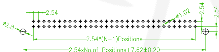
△ Recommended PCB Layout (PCB TOLERANCE ±0.05)
