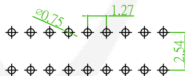
Recommended PCB Layout (PCB TOLERANCE \pm 0.1 )
