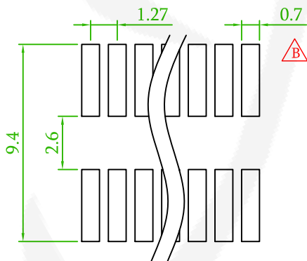
Recommended PCB Layout (PCB TOLERANCE ±0.1)
