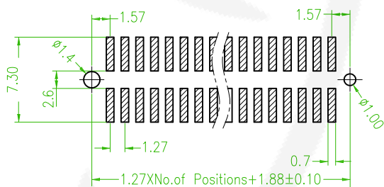
Recommended PCB Layout (PCB TOLERANCE ±0.1)
