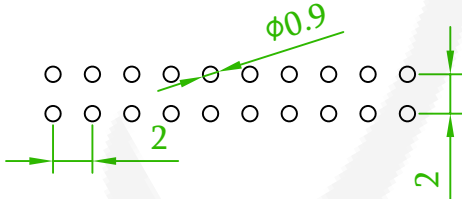
Recommended PCB Layout (PCB TOLERANCE ±0.1)
