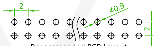
Recommended PCB Layout (PCB TOLERANCE ±0.1)
