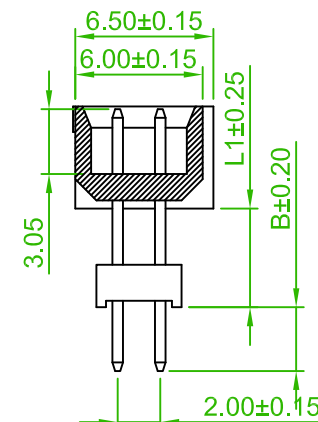
SECTION A-A Old Part No.:BH2EGS-XX-U
