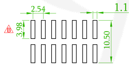
Recommended PCB Layout (PCB TOLERANCE ±0.1)
