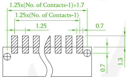
P.C.B. LAYOUT TOLERANCE: ± 0.1
