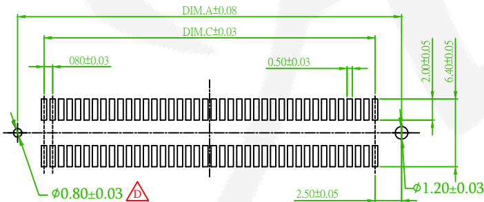
Recommended PCB Layout (PCB TOLERANCE ±0.05)
