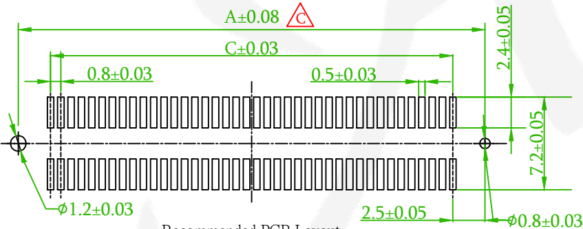
Recommended PCB Layout (PCB TOLERANCE ±0.05)
