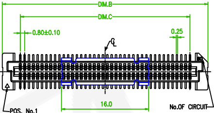
△E 5BB085C38F-XXXXXUR-01
