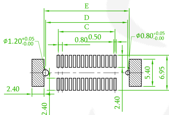
Recommended PCB Layout (PCB TOLERANCE \pm 0.05 )
